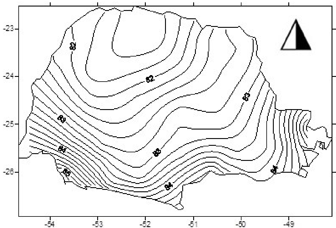
Figure 7 - 50.0 % of the precipitation (CI = 1.0 mm).
