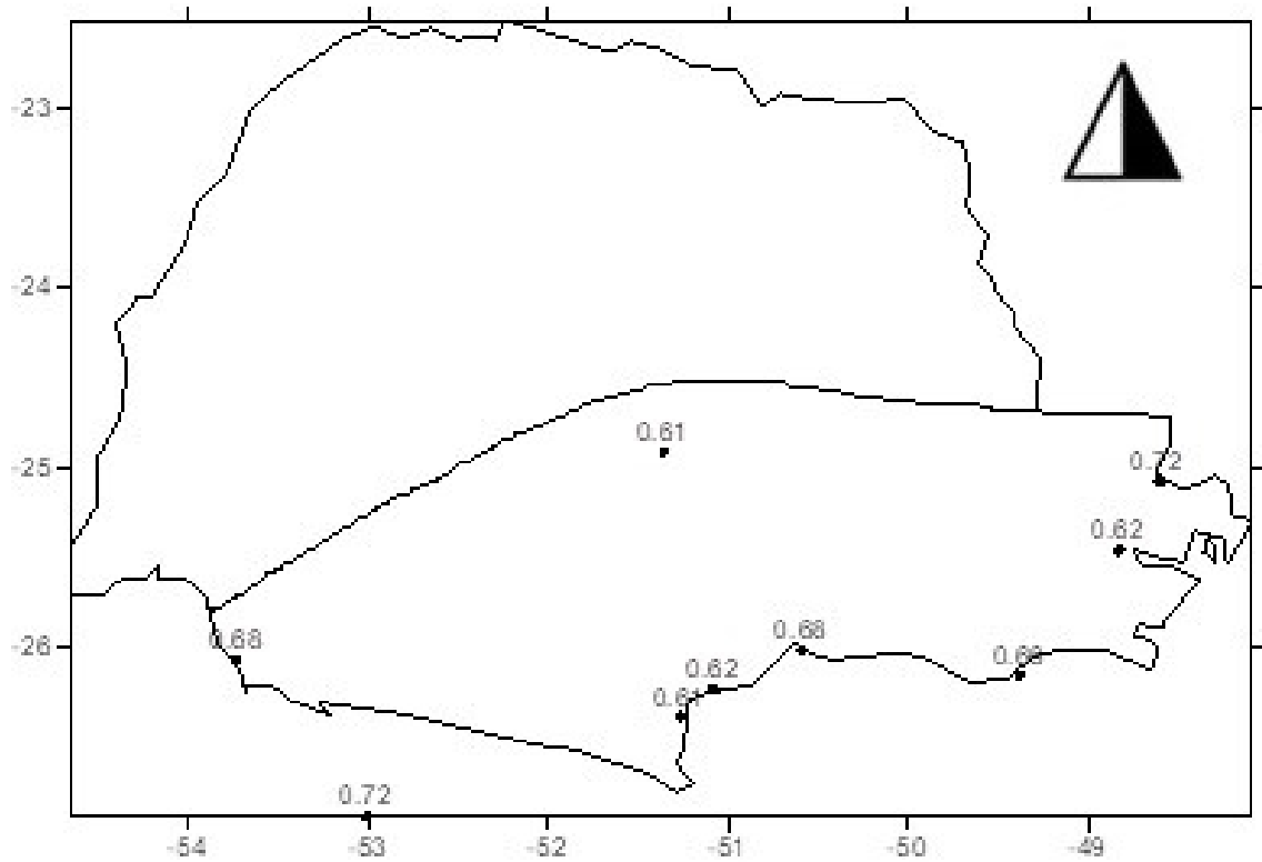
Figure 3 - CI values greater than 0.60.
