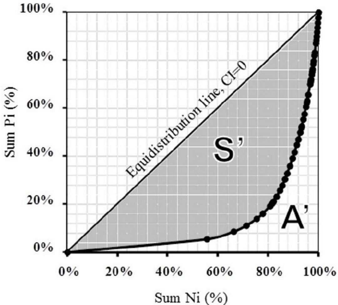
Figure 2 - Exponential curve of the number of precipitation days (Sum Ni) versus accumulated rainfall (Sum Pi). The solid black line is the equidistribution line.
