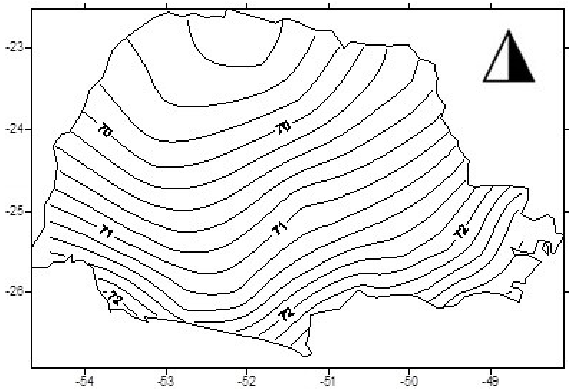
Figure 6 - 30.0 % of the precipitation (CI = 1.0 mm).
