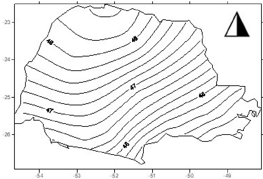
Figure 4 - 10.0 % of the precipitation (CI = 1.0 mm).
