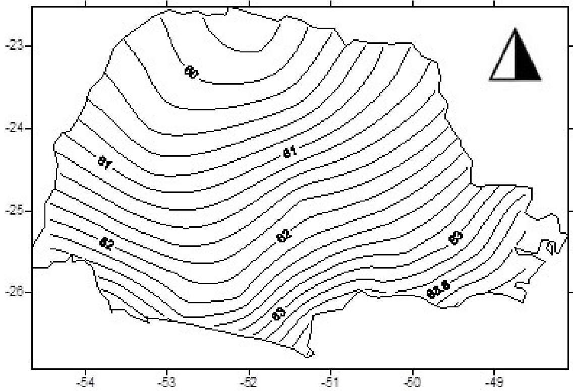
Figure 5 - 20.0 % of the precipitation (CI = 1.0 mm).
