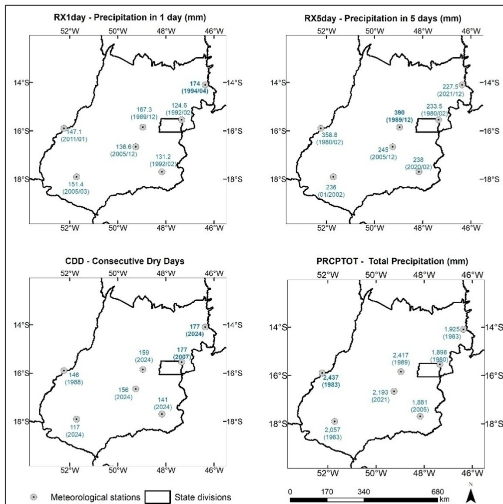
Figure 3 – Spatial variation of extreme events from 1980 to 2024 for some indices associated with precipitation (RX1day, RX5day, CDD and PRCPOT). Source: authors, based on INMET data processed in RCLIMDEX.
