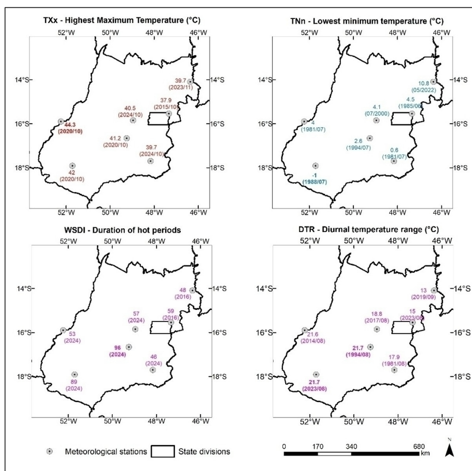
Figure 2 – Spatial variation of extreme events from 1980 to 2024 for some indices associated with air temperature (TXx, TNn, WSDI and DTR). Source: authors, based on INMET data processed in RCLimDEX.
